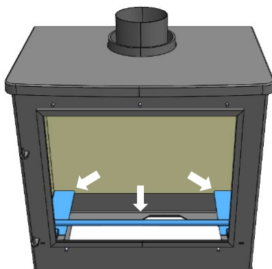
Fig.2 Remove front bar and mesh trims
