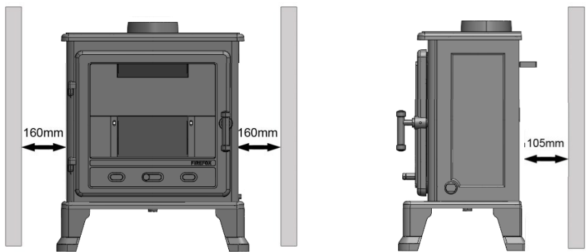
Fig.5 Clearances
