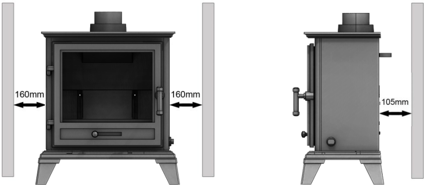
Fig.5 Clearances
