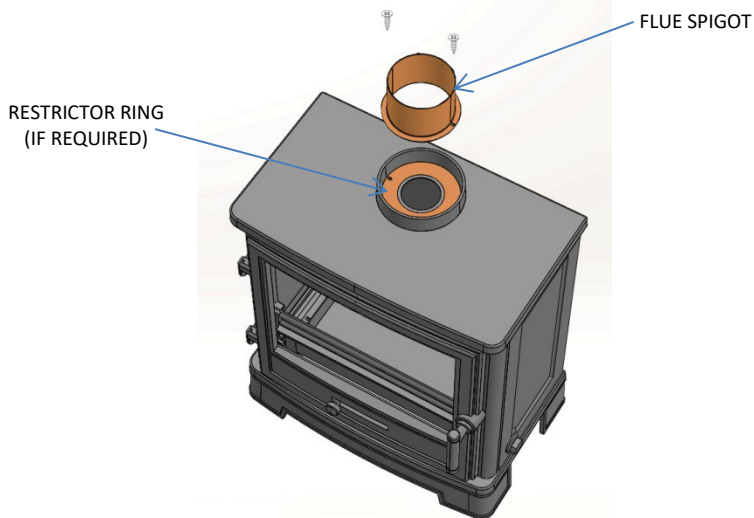
Fig.7 Flue connections
